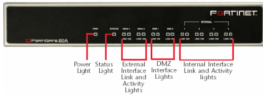
FortiGate-100A
